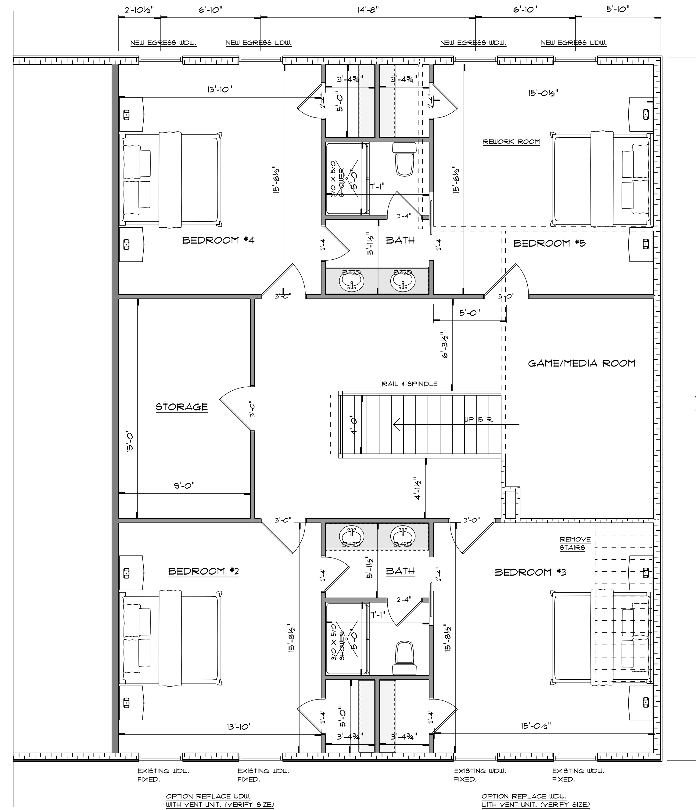
SECOND FLOOR SCALE: 1/4" = 1'-0"
